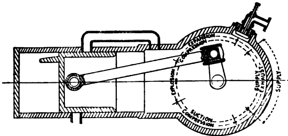
FIG. 280.—Diagram of the stages of a Two-Part Cycle Gas Engine. The out-stroke is from left to right; the in-stroke from right to left. The inner circle around the crank case in front of the piston. The outer circle shows the stages of explosion, expansion, exhaust and compression, which take place behind the piston in the combustion space of the cylinder.
